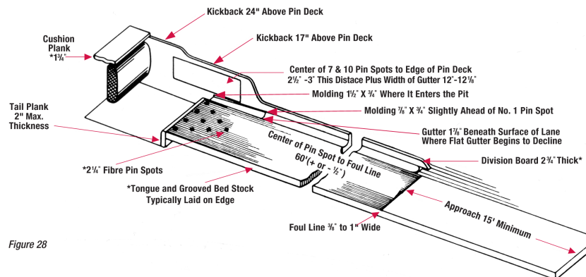
USBC Regulation Bowling Lane Dimensions Typical Cross Section of Bowling Lane — Round Gutters from foul line to pin deck area.
